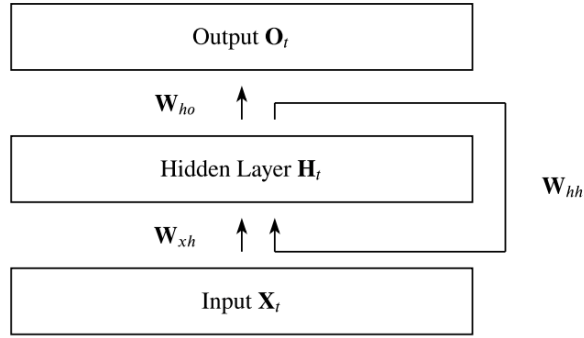
Figure 3.6 Basic illustration of the recurrent neural networks [57].
