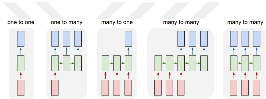
Figure 3.10 Illustration of various types of data and tasks [64].
