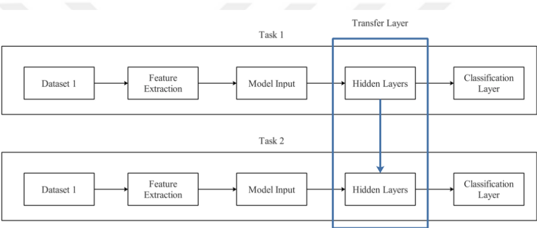
Figure 3.8 Schematic diagram of a transfer learning model: The first phase involves training with Task 1, followed by training a new model for Task 2 that leverages the knowledge acquired from the model developed for Task 1 [63].
