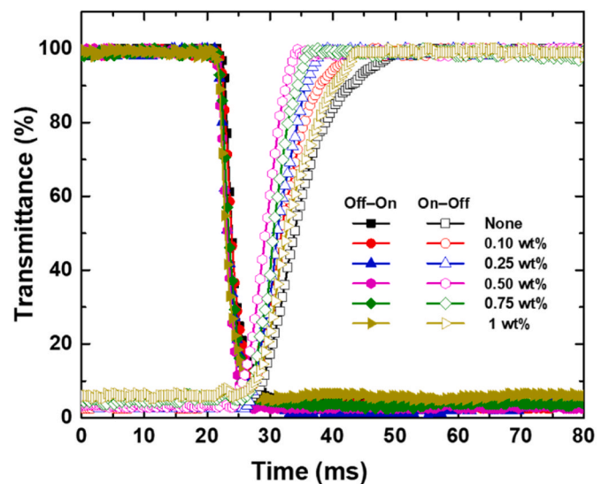
Fig. 6. Time-dependent optical transmittance for TN LC cells containing varied concentrations of ZnCdTeS QDs at 25 °C.
