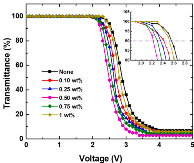
Fig. 5. Voltage-dependent optical transmittance for TN LC samples containing varied concentrations of ZnCdTeS QDs at 50 Hz and the temperature of 25 °C. The inset displays an expanded view of V-T curves close to the transmittance of 90%.
