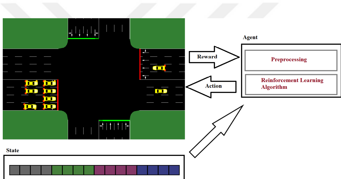
Figure 3.1 Visualization on how a generic Reinforcement Learning algorithm would work on a traffic light environment
