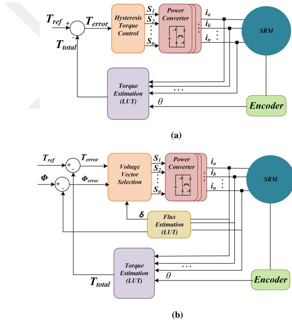
Figure 3. 11 (a) DITC Block Diagram and (b) DTC block diagram.
