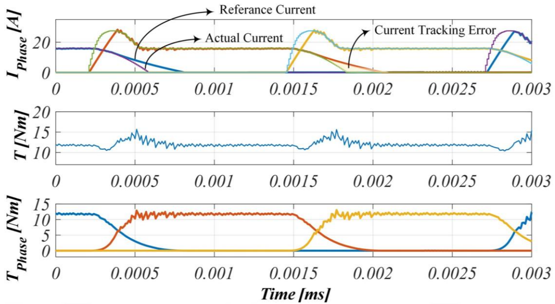
Figure 5. 8 Simulation result Cubic TSF at 1000 rpm.
