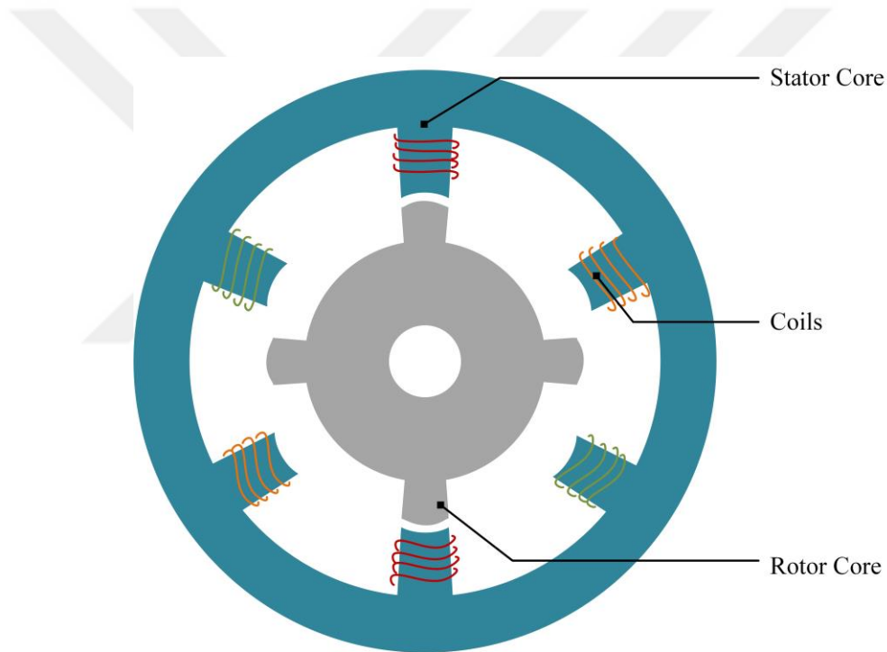
Figure 3. 1 Structure of the SRM.
