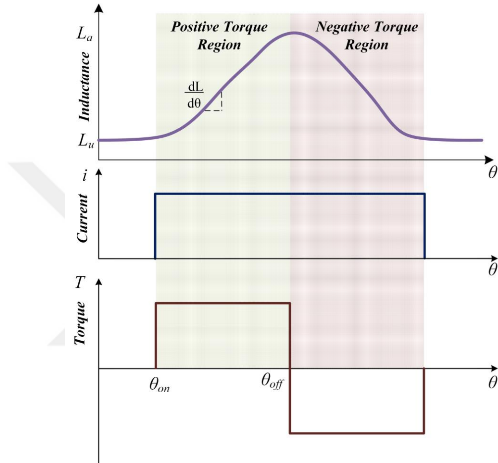
Figure 3. 5 Idealized inductance, current, and torque profile.
