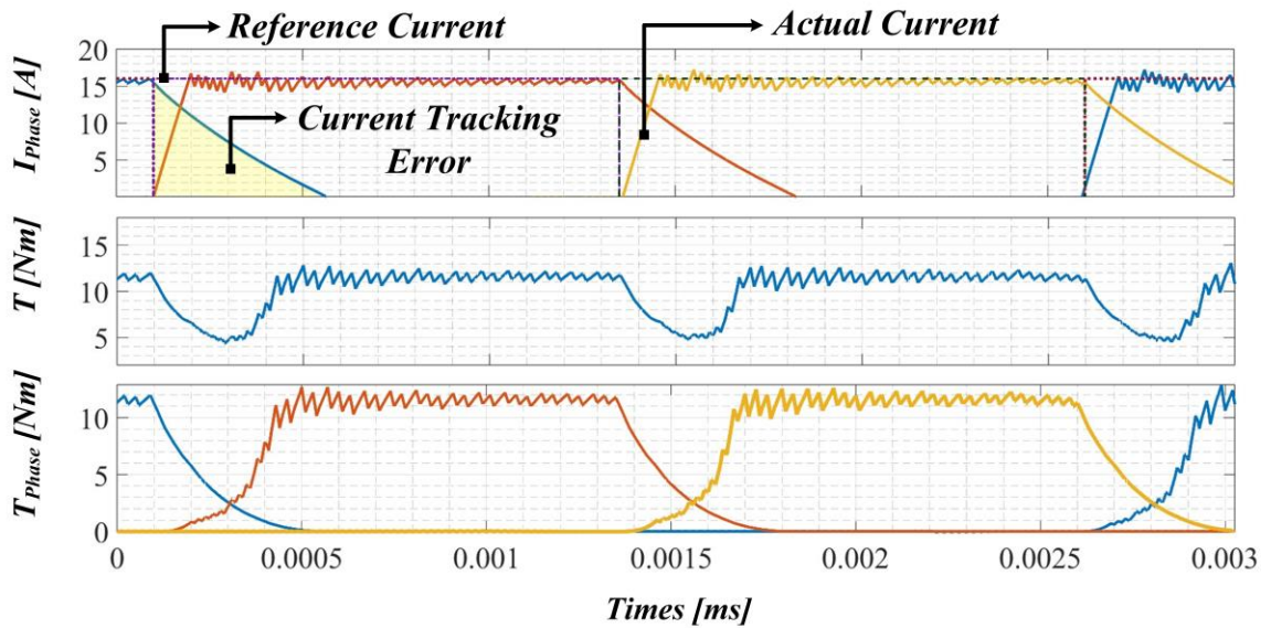
Figure 5. 6 Hysteresis current control behavior for SRM.
