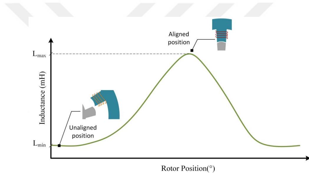
Figure 3. 2 Inductance variation profile in the SRM.
