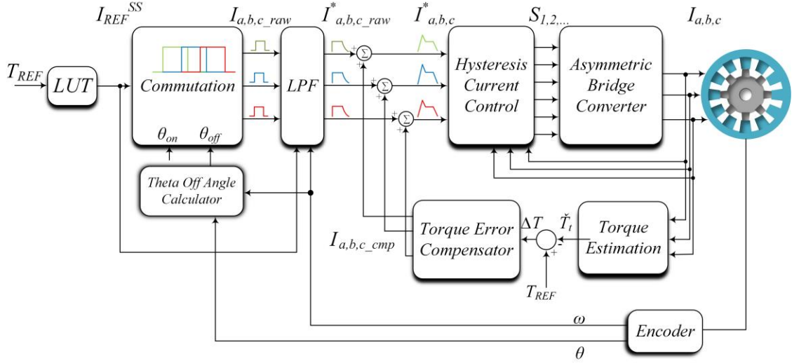
Figure 4. 2 Proposed control algorithm for SRM.
