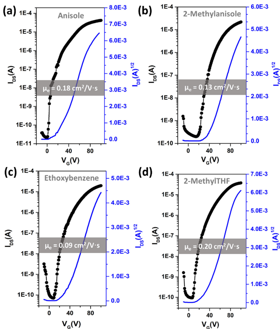
Fig. 4 Transfer plots ( V_{DS} = 100 V) for the fabricated OFET devices of \beta,\beta' -C 12 -TTFDMT on p ++ -Si/SiO 2 /PS-brush ( M_n = 5 kDa) spin-coated from anisole (a), 2-methylanisole (b), ethoxybenzene (c), and 2-methyltetrahydrofuran (d) solutions. All measurements were performed under ambient conditions, and the electron mobilities were based on the transfer curves shown herein.
