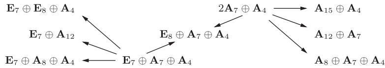
FIGURE 1. The graph \mathfrak{C}_2 .
