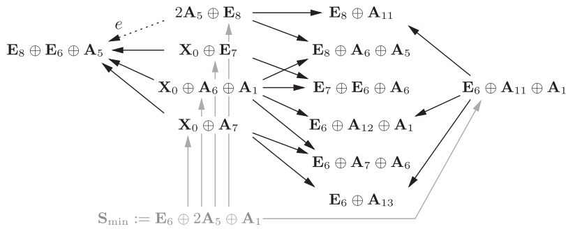
FIGURE 2. The graph \mathcal{C}_3 (where \mathbf{X}_0 := \mathbf{E}_6 + \mathbf{A}_5 ).
