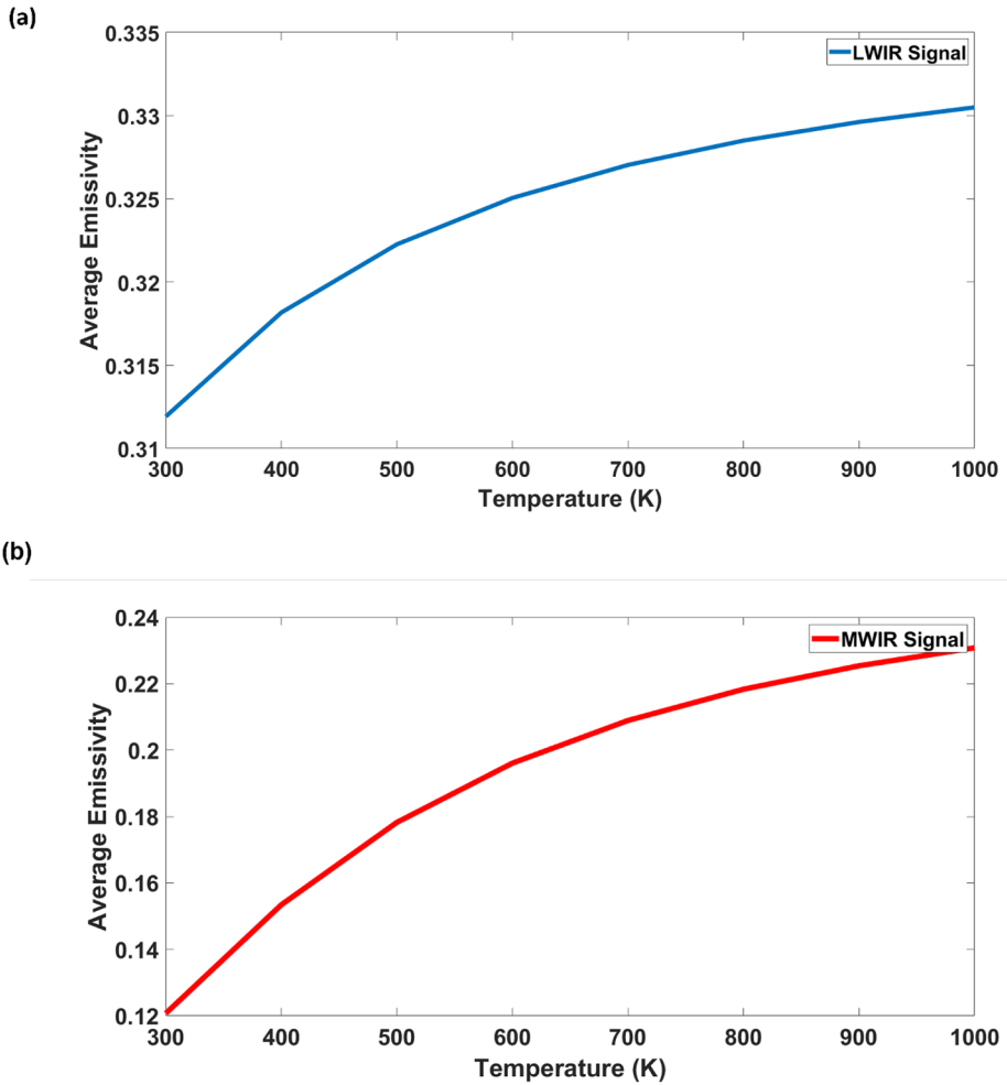
Fig. 6 (a), (b). MWIR and LWIR signature analysis of DNE by calculating its average thermal emission
