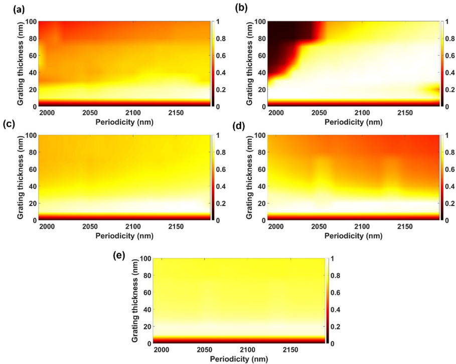
Fig. 3 (a–e) Contour plots of the dual parameter sweep analysis of designed DNE calculated for various grating thickness t against periodicity P for given wavelengths \lambda_1 , \lambda_2 , \lambda_3 , \lambda_4 , and \lambda_5 respectively. Color bars represent the absorption
