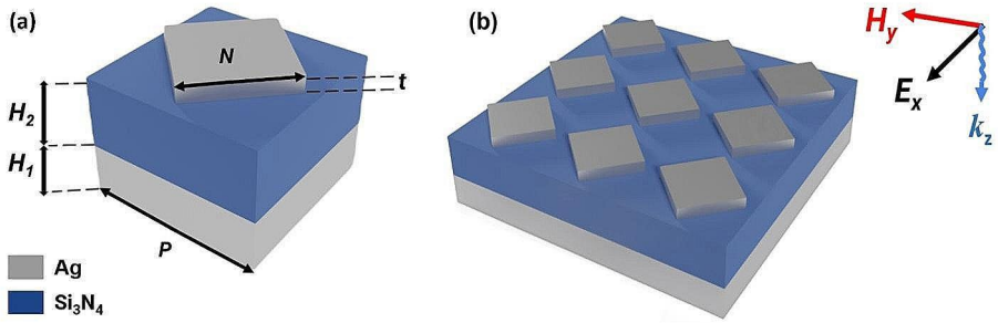
Fig. 1 Schematic design of the presented nanoantenna. (a) Perspective view of the presented nanoantenna unit cell, (b) 3D view of the nanoantenna array sheet
