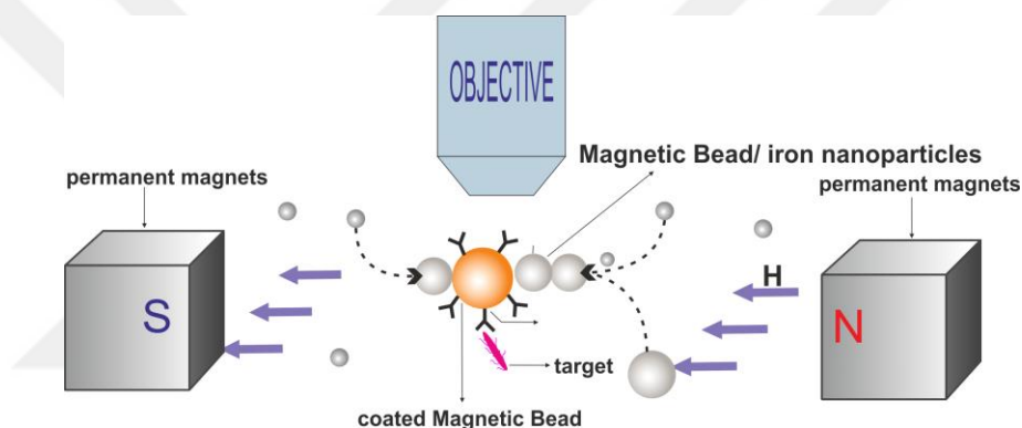
Figure 1.3.1 Demonstration of the experimental setup and magnetic beads accumulation based signal amplification
