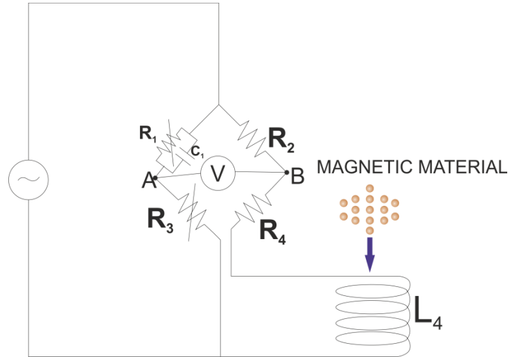
Figure 1.2.4.2 Maxwell's bridge setup
