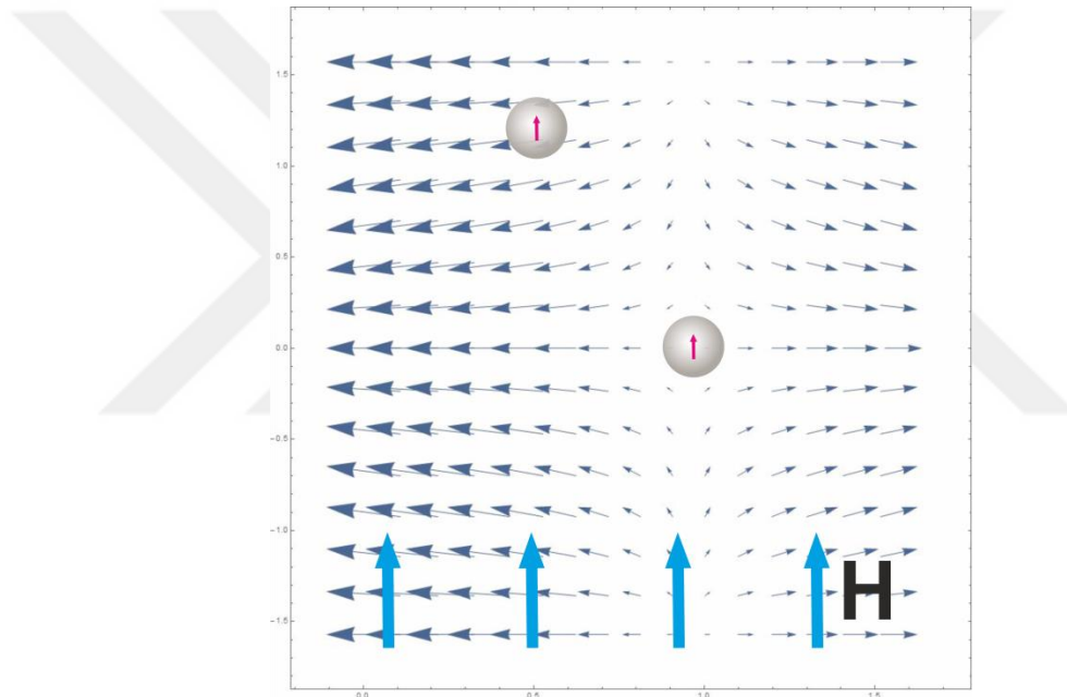
Figure 2.3.2 Normalized dipole-dipole force field
