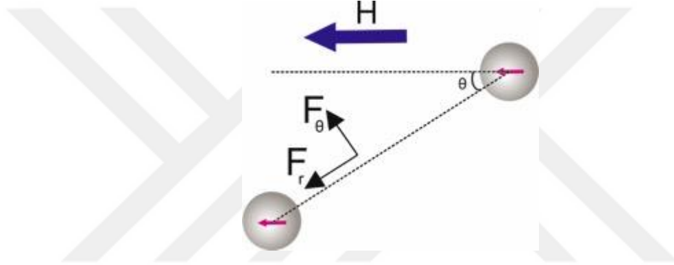
Figure 2.3.1 Diagram showing the positions of the interacting magnetic beads and the magnetic fields direction
