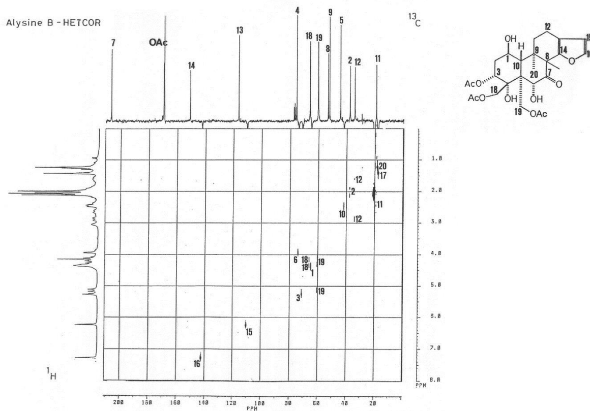
Figure S8. 1 H- 13 C correlation (HETCOR) spectrum of alysine B.
